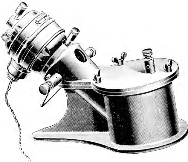
FIG. 18.—Improved Mackenzie Davidson interrupter. (Schall.)
